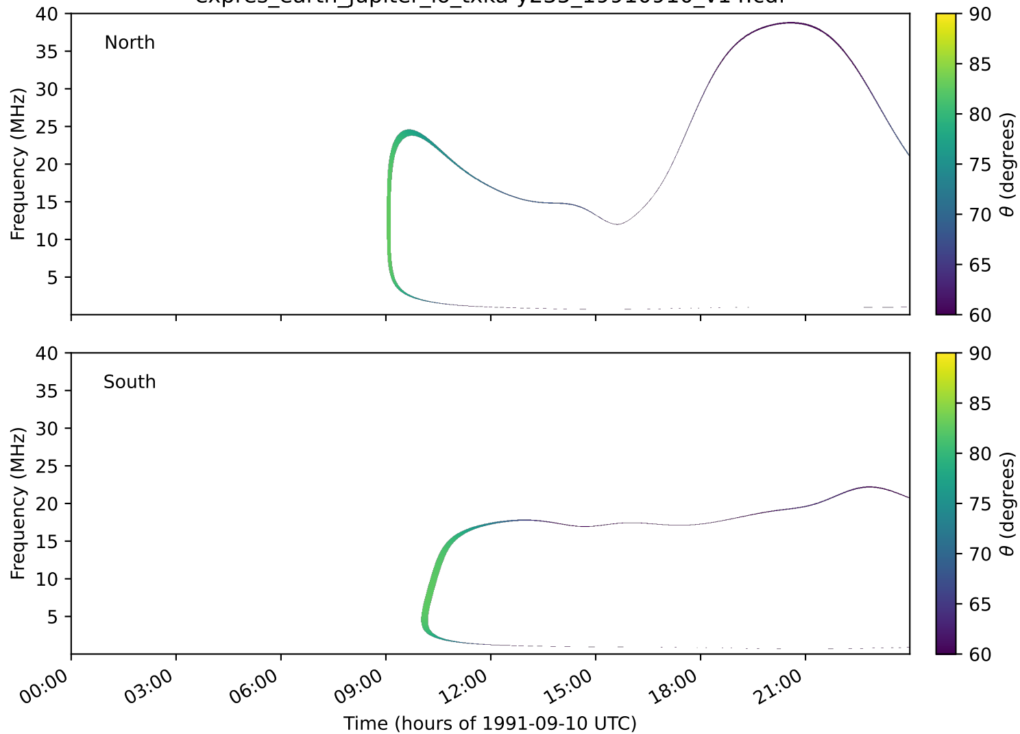
expres_earth_jupiter_io_txka-y235_19910910_v14.cdf
