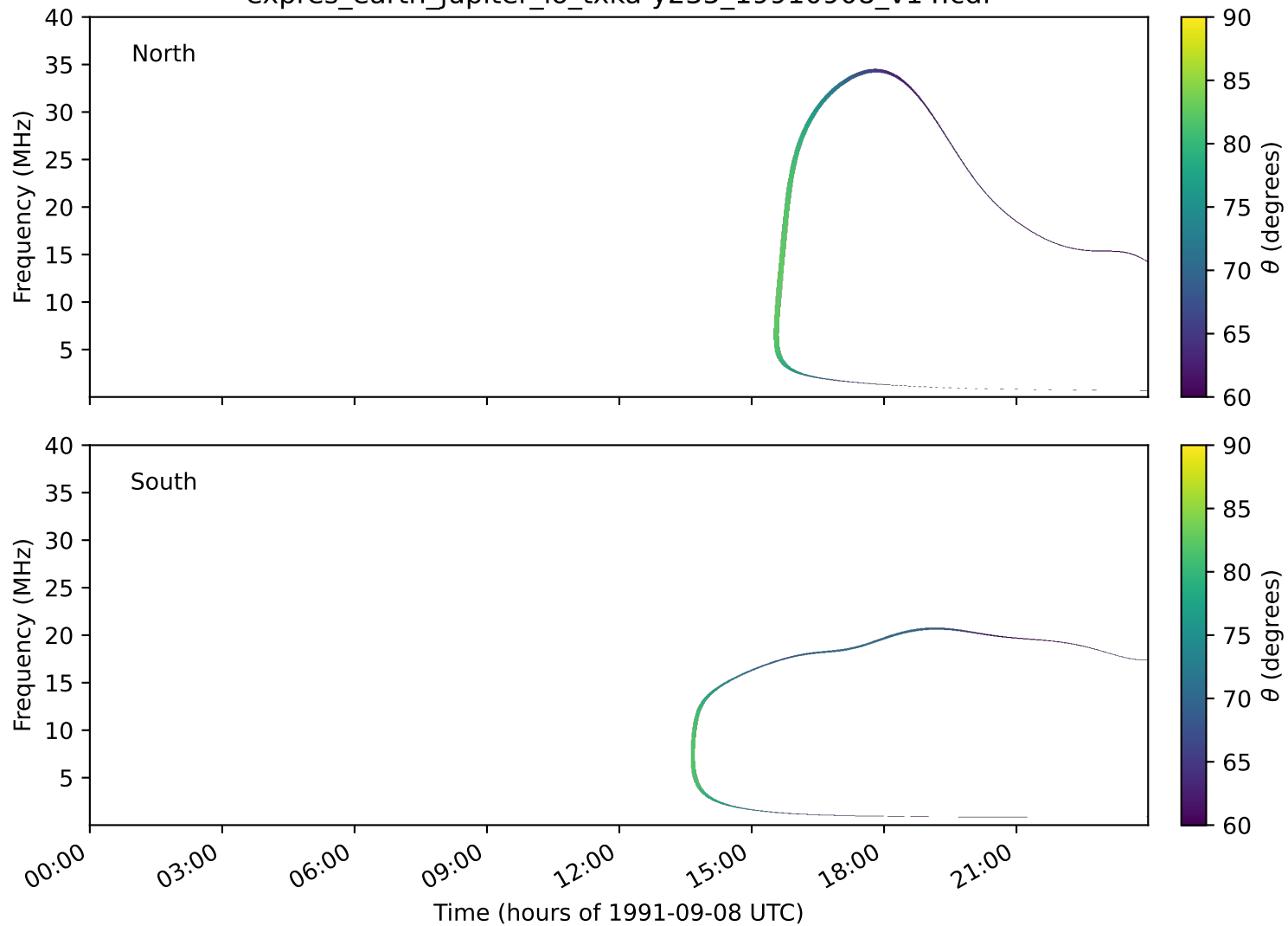
expres_earth_jupiter_io_txka-y235_19910908_v14.cdf
