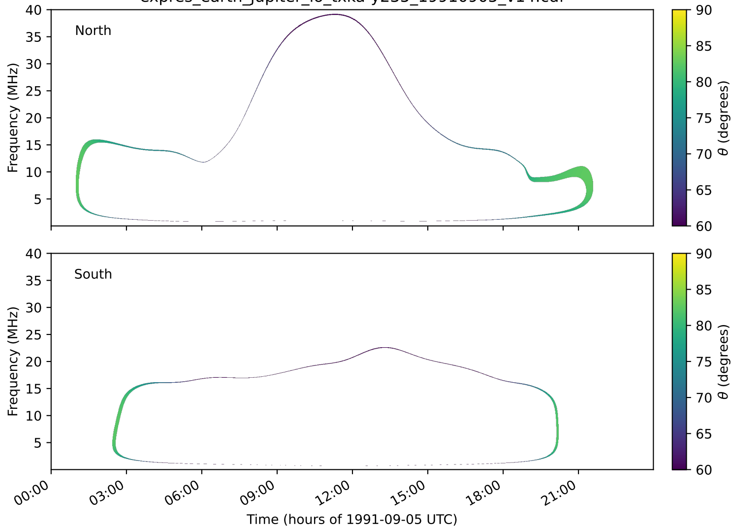
expres_earth_jupiter_io_txka-y235_19910905_v14.cdf
