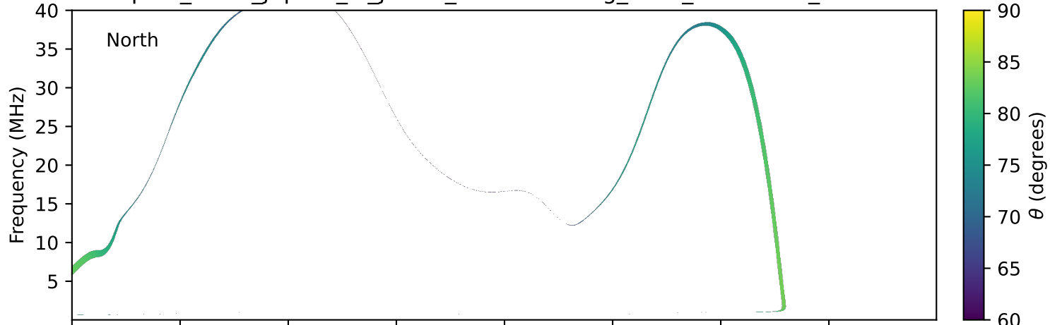
expres_earth_jupiter_io_jrm33_lossc-wid1deg_3kev_19910930_v11.cdf
