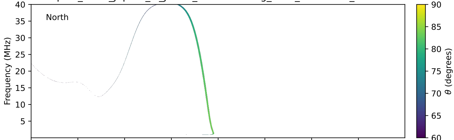
expres_earth_jupiter_io_jrm33_lossc-wid1deg_3kev_19910925_v11.cdf
