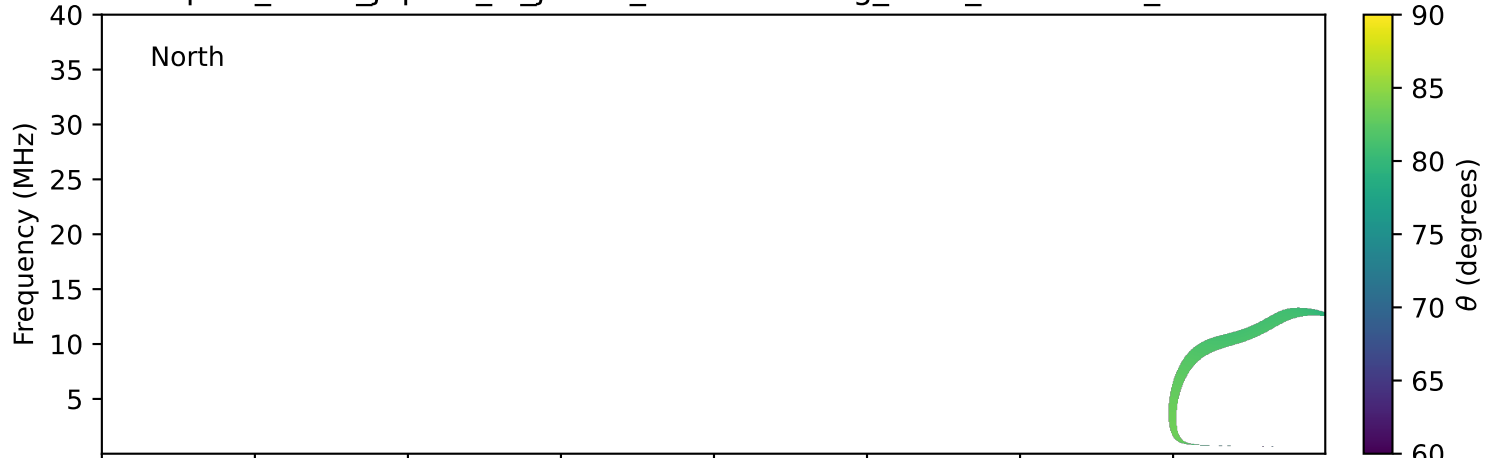
expres_earth_jupiter_io_jrm33_lossc-wid1deg_3kev_19910922_v11.cdf
