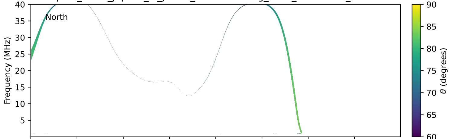
expres_earth_jupiter_io_jrm33_lossc-wid1deg_3kev_19910914_v11.cdf
