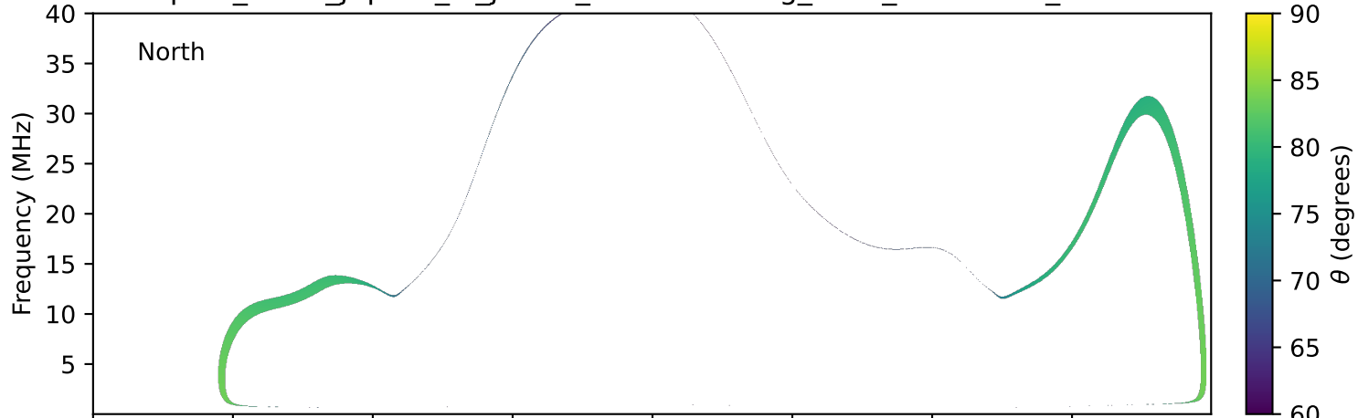
expres_earth_jupiter_io_jrm33_lossc-wid1deg_3kev_19910912_v11.cdf
