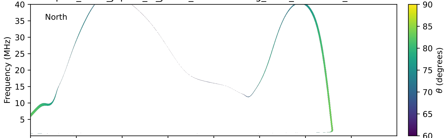
expres_earth_jupiter_io_jrm09_lossc-wid1deg_3kev_19910930_v11.cdf
