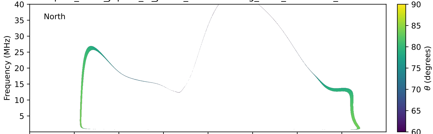
expres_earth_jupiter_io_jrm09_lossc-wid1deg_3kev_19910921_v11.cdf
