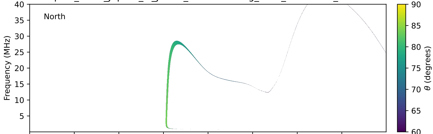
expres_earth_jupiter_io_jrm09_lossc-wid1deg_3kev_19910910_v11.cdf
