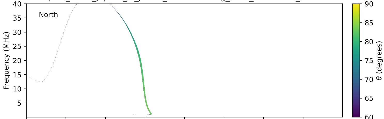
expres_earth_jupiter_io_jrm09_lossc-wid1deg_3kev_19910909_v11.cdf
