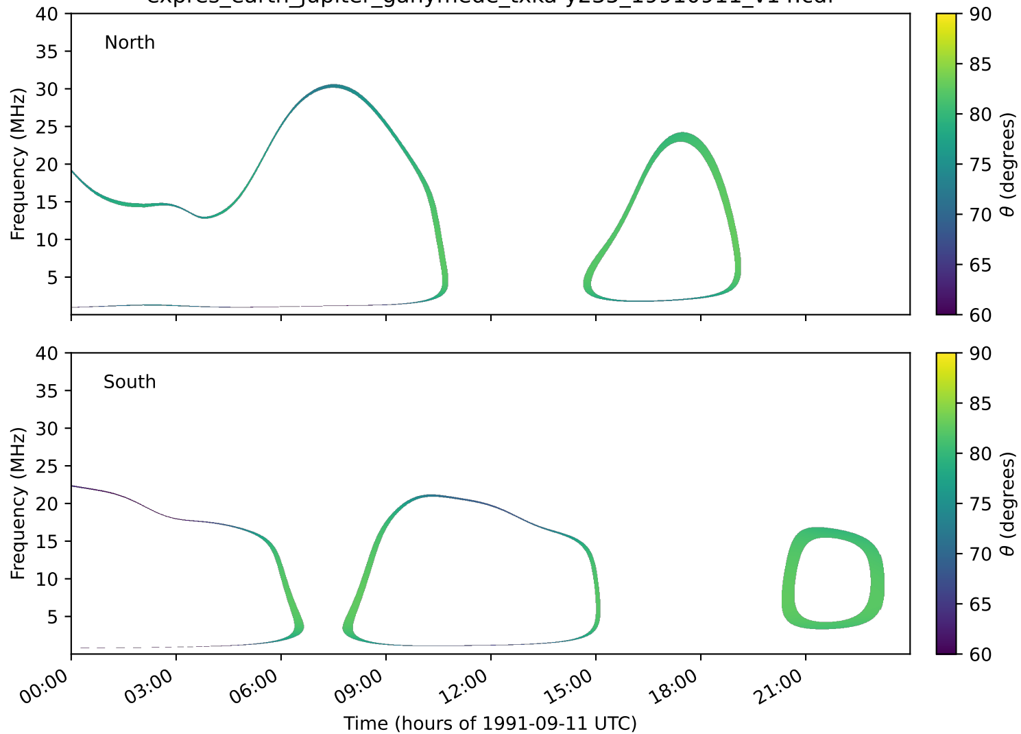
expres_earth_jupiter_ganymede_txka-y235_19910911_v14.cdf
