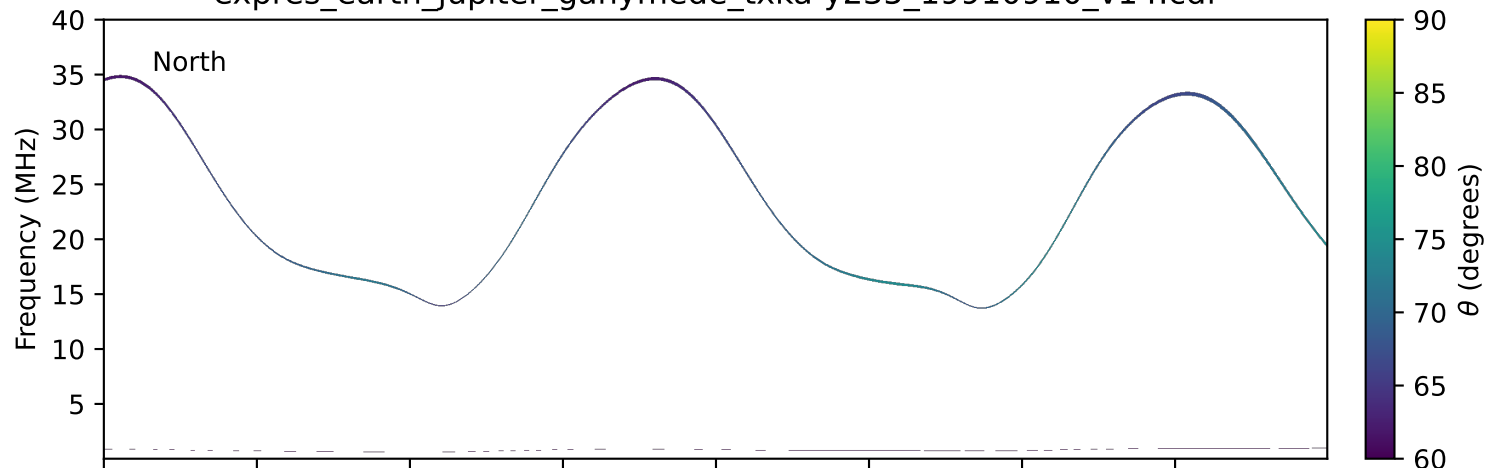
expres_earth_jupiter_ganymede_txka-y235_19910910_v14.cdf
