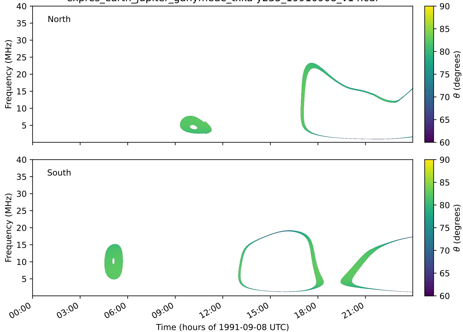
expres_earth_jupiter_ganymede_txka-y235_19910908_v14.cdf
