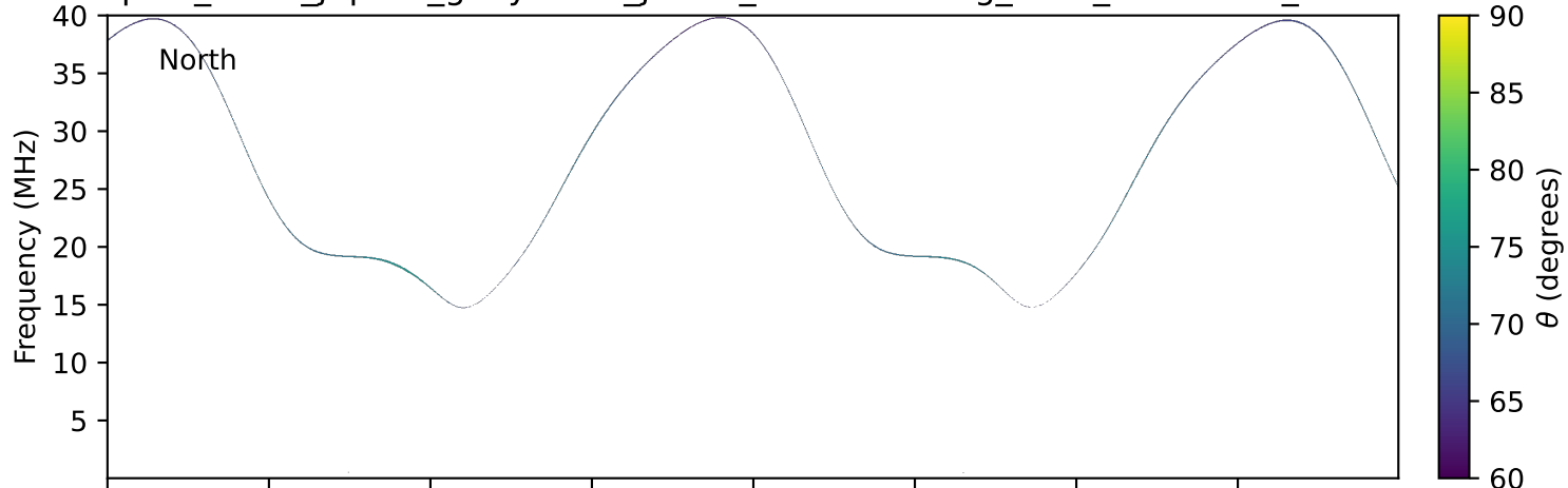
expres_earth_jupiter_ganymede_jrm33_lossc-wid1deg_3kev_19910917_v11.cdf
