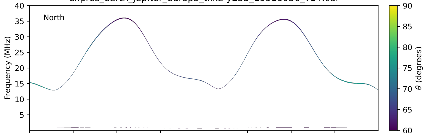
expres_earth_jupiter_europa_txka-y235_19910930_v14.cdf
