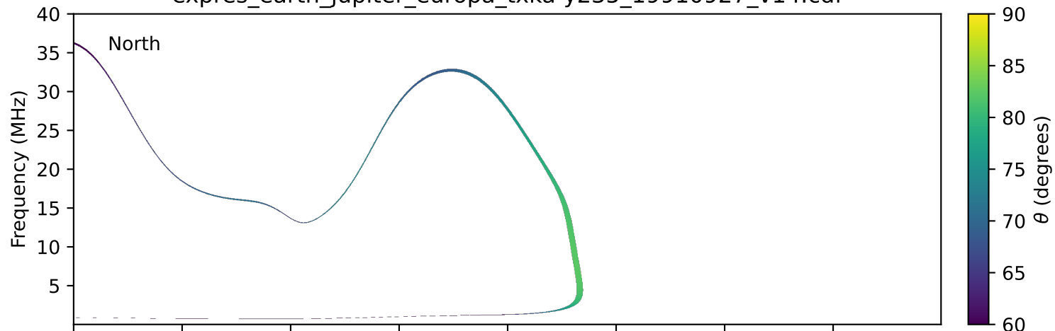
expres_earth_jupiter_europa_txka-y235_19910927_v14.cdf
