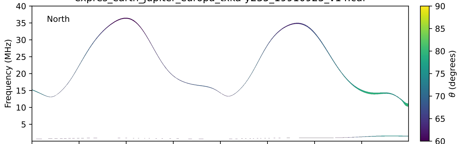
expres_earth_jupiter_europa_txka-y235_19910923_v14.cdf
