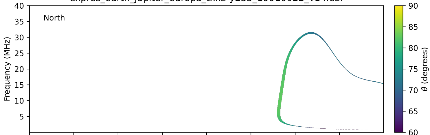
expres_earth_jupiter_europa_txka-y235_19910922_v14.cdf
