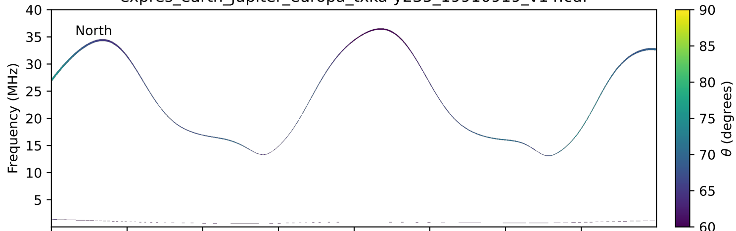
expres_earth_jupiter_europa_txka-y235_19910919_v14.cdf
