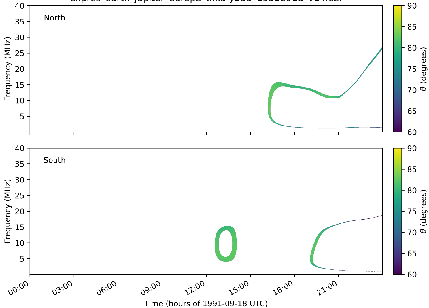
expres_earth_jupiter_europa_txka-y235_19910918_v14.cdf
