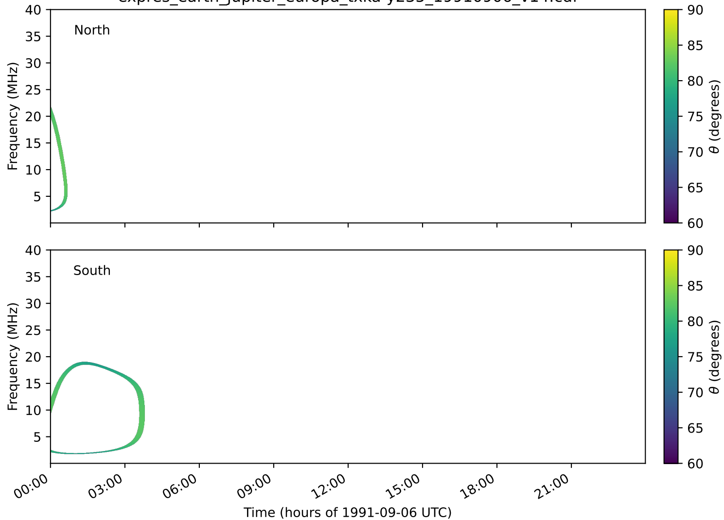
expres_earth_jupiter_europa_txka-y235_19910906_v14.cdf
