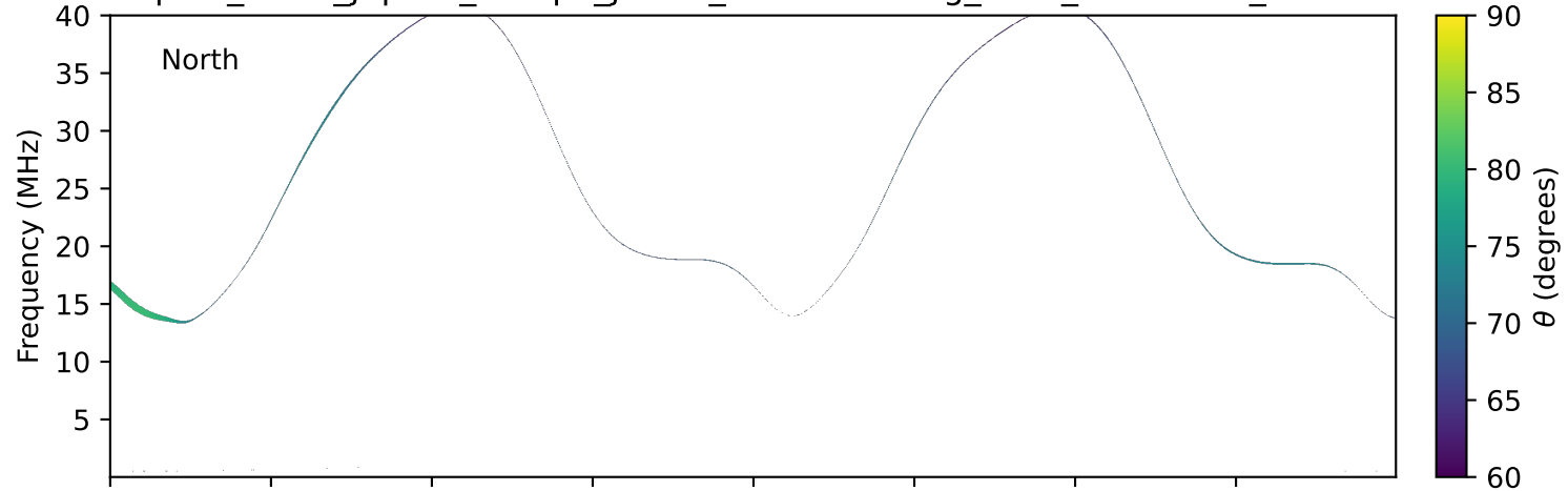
expres_earth_jupiter_europa_jrm33_lossc-wid1deg_3kev_19910930_v11.cdf
