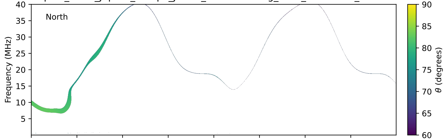
expres_earth_jupiter_europa_jrm33_lossc-wid1deg_3kev_19910901_v11.cdf
