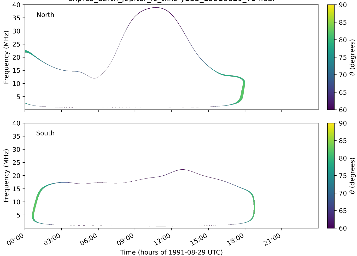
expres_earth_jupiter_io_txka-y235_19910829_v14.cdf
