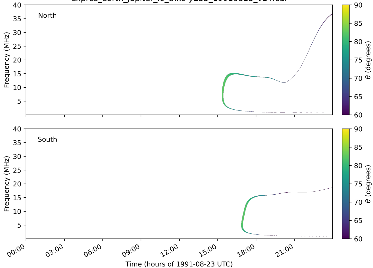
expres_earth_jupiter_io_txka-y235_19910823_v14.cdf
