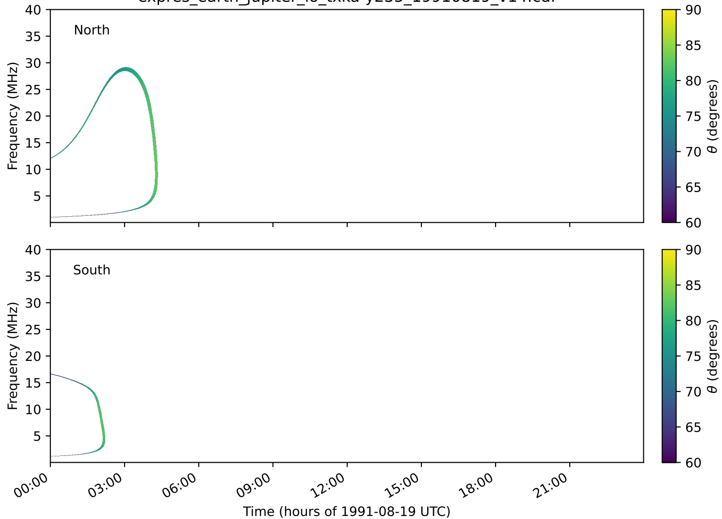
expres_earth_jupiter_io_txka-y235_19910819_v14.cdf
