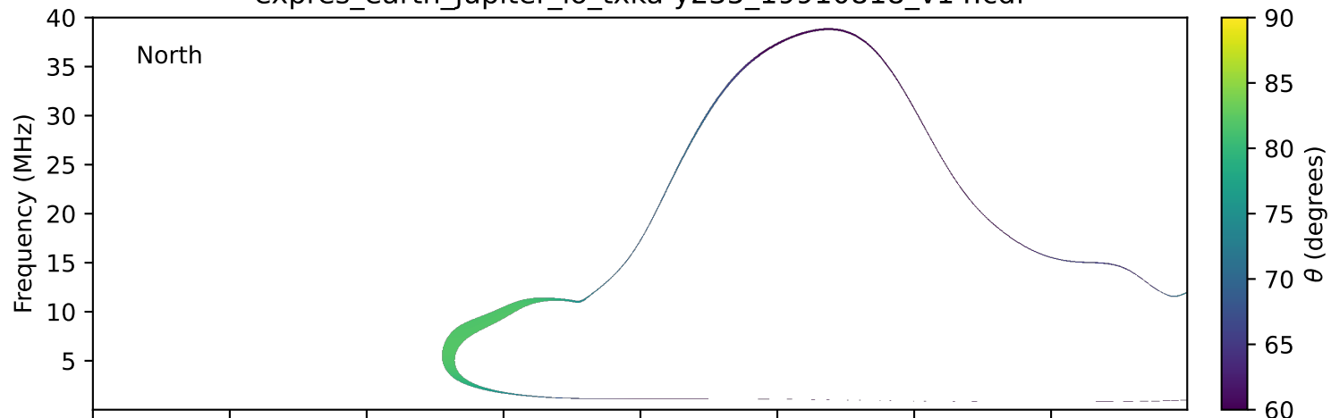
expres_earth_jupiter_io_txka-y235_19910818_v14.cdf
