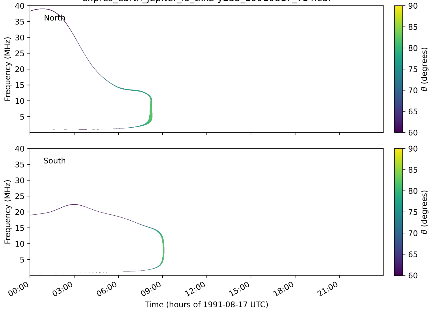
expres_earth_jupiter_io_txka-y235_19910817_v14.cdf
