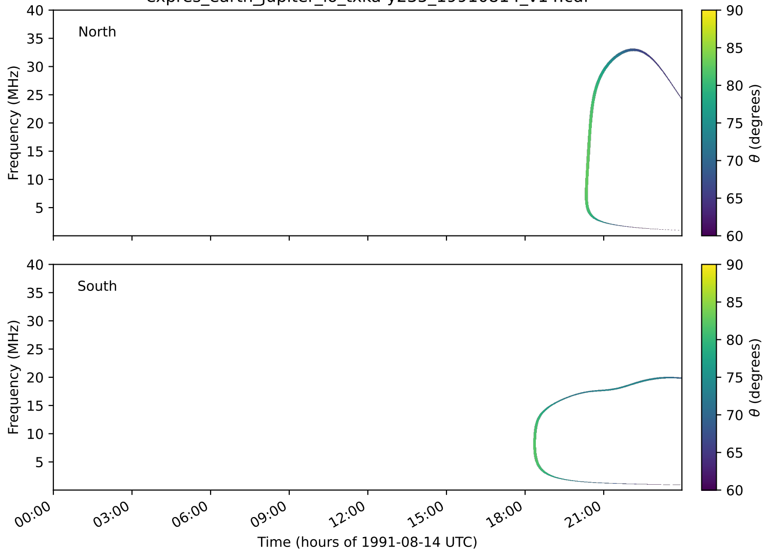
expres_earth_jupiter_io_txka-y235_19910814_v14.cdf
