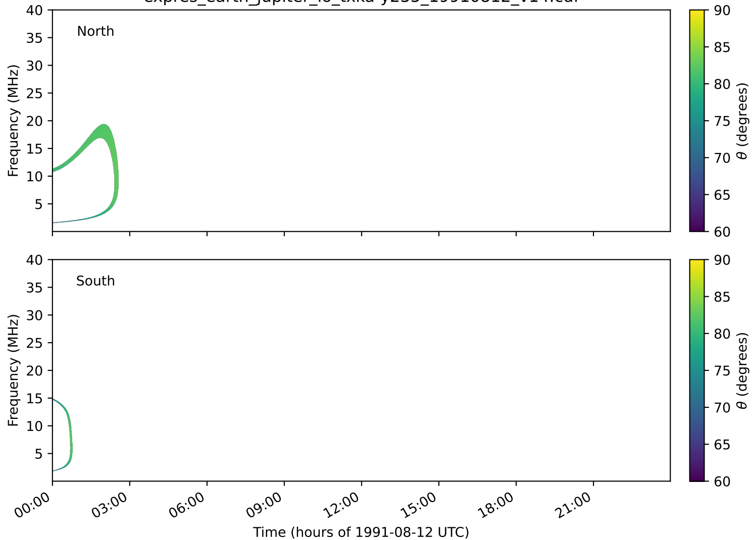
expres_earth_jupiter_io_txka-y235_19910812_v14.cdf
