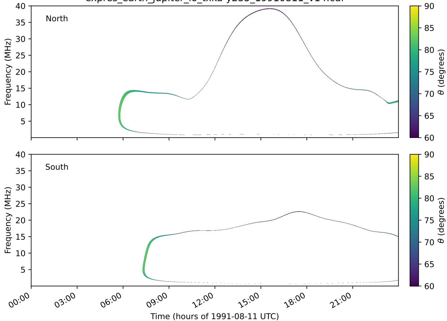
expres_earth_jupiter_io_txka-y235_19910811_v14.cdf
