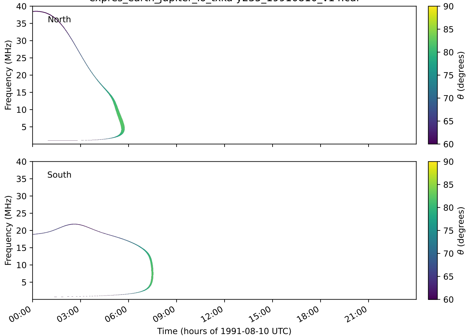
expres_earth_jupiter_io_txka-y235_19910810_v14.cdf
