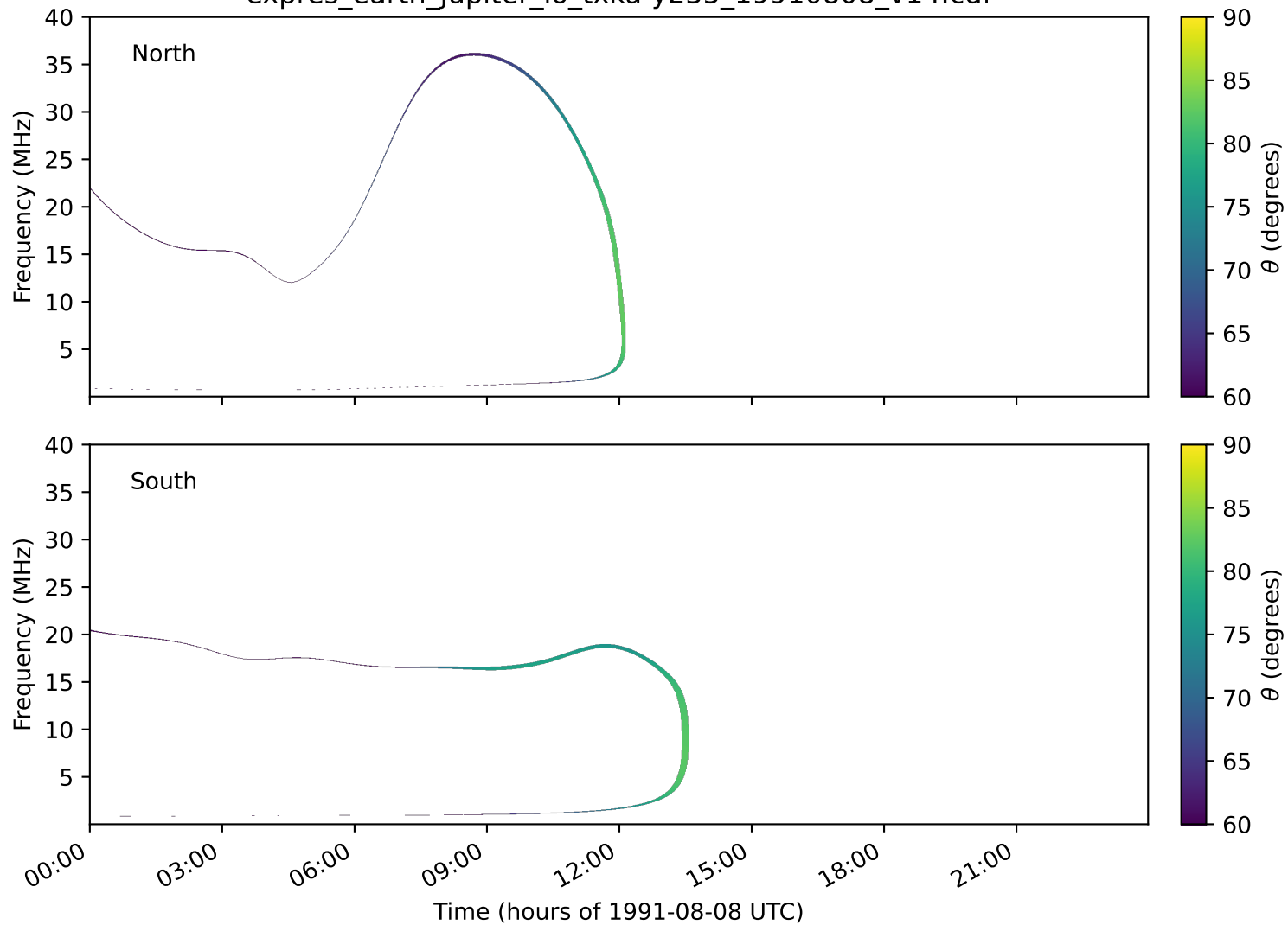
expres_earth_jupiter_io_txka-y235_19910808_v14.cdf
