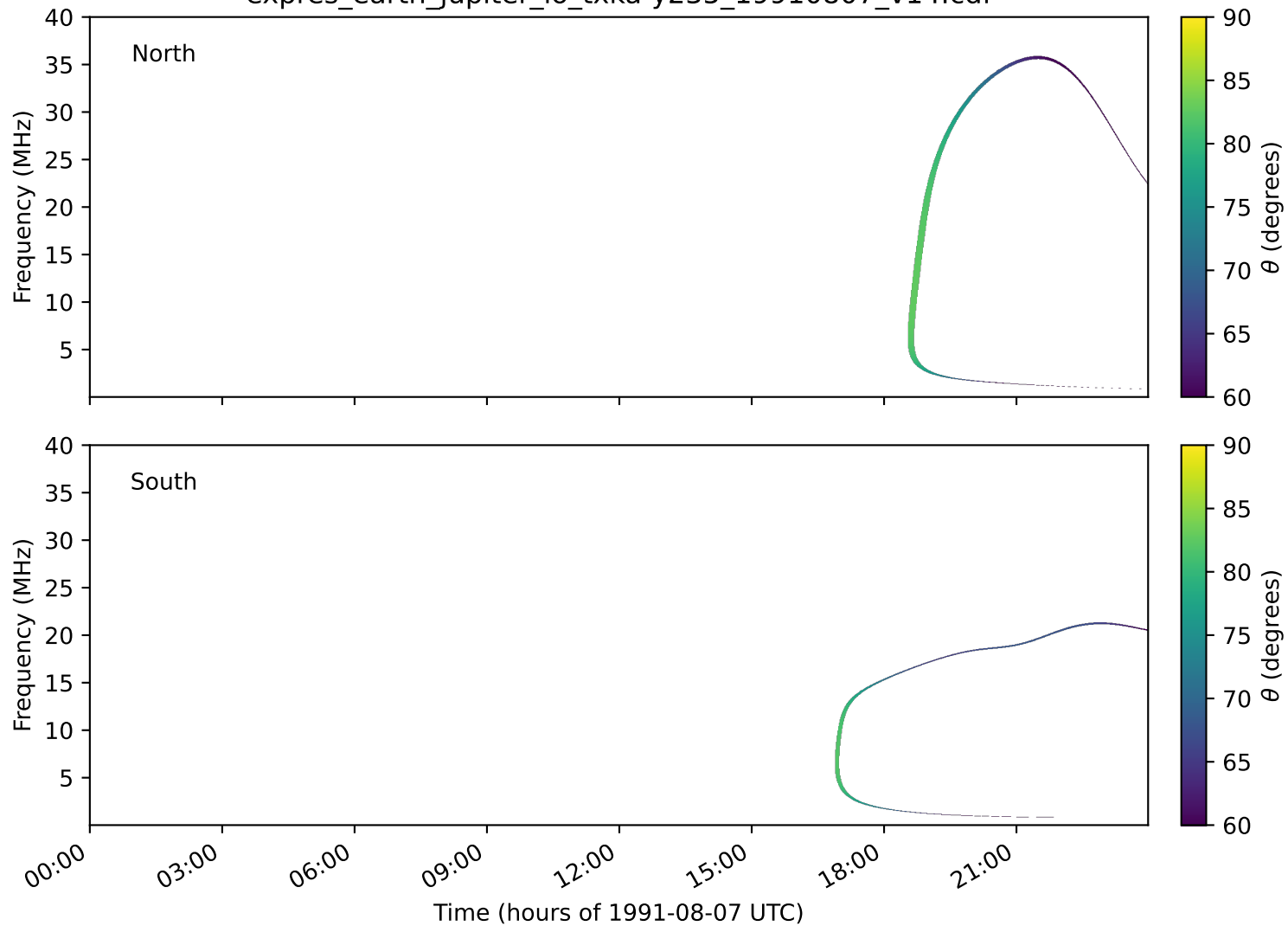
expres_earth_jupiter_io_txka-y235_19910807_v14.cdf
