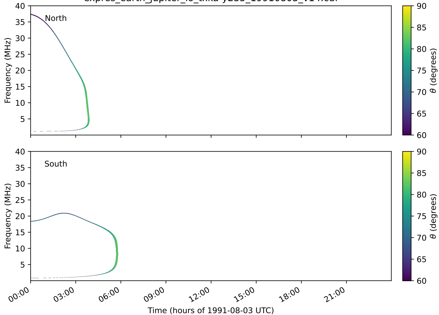
expres_earth_jupiter_io_txka-y235_19910803_v14.cdf
