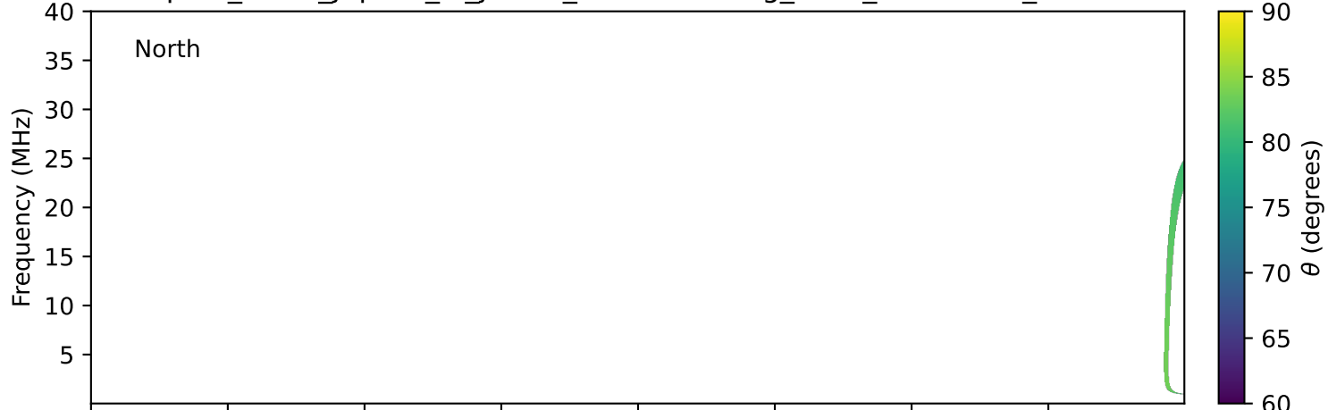
expres_earth_jupiter_io_jrm33_lossc-wid1deg_3kev_19910828_v11.cdf
