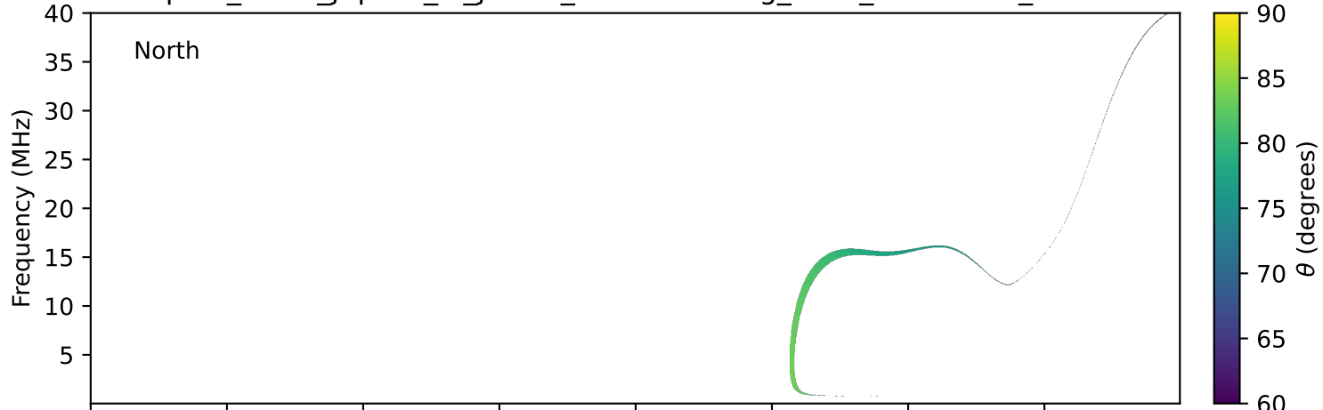
expres_earth_jupiter_io_jrm33_lossc-wid1deg_3kev_19910823_v11.cdf
