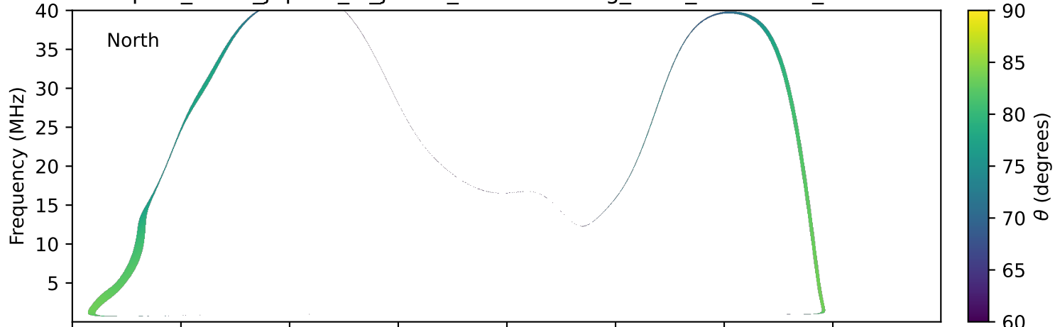
expres_earth_jupiter_io_jrm33_lossc-wid1deg_3kev_19910813_v11.cdf
