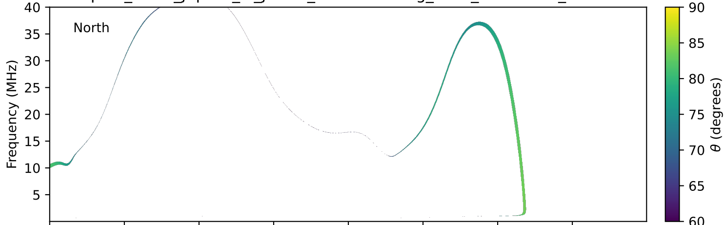
expres_earth_jupiter_io_jrm33_lossc-wid1deg_3kev_19910806_v11.cdf
