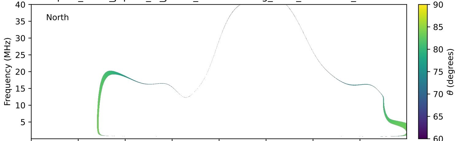
expres_earth_jupiter_io_jrm33_lossc-wid1deg_3kev_19910804_v11.cdf
