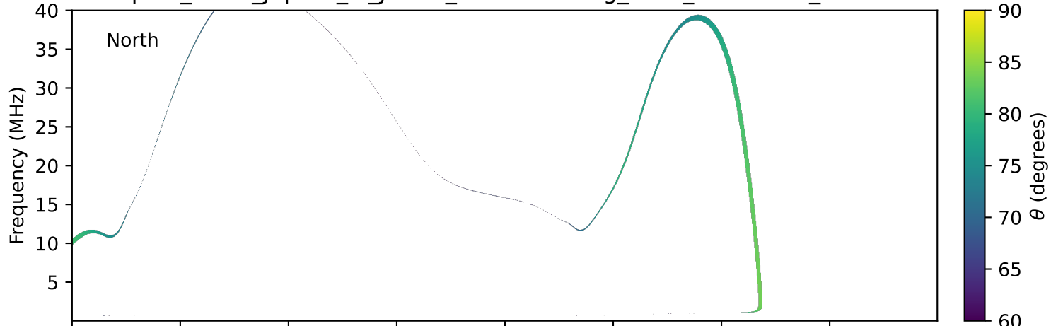
expres_earth_jupiter_io_jrm09_lossc-wid1deg_3kev_19910806_v11.cdf
