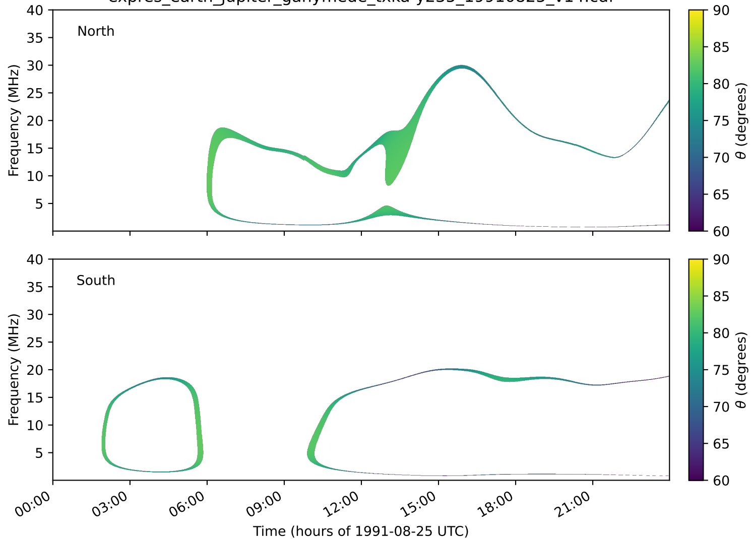
expres_earth_jupiter_ganymede_txka-y235_19910825_v14.cdf
