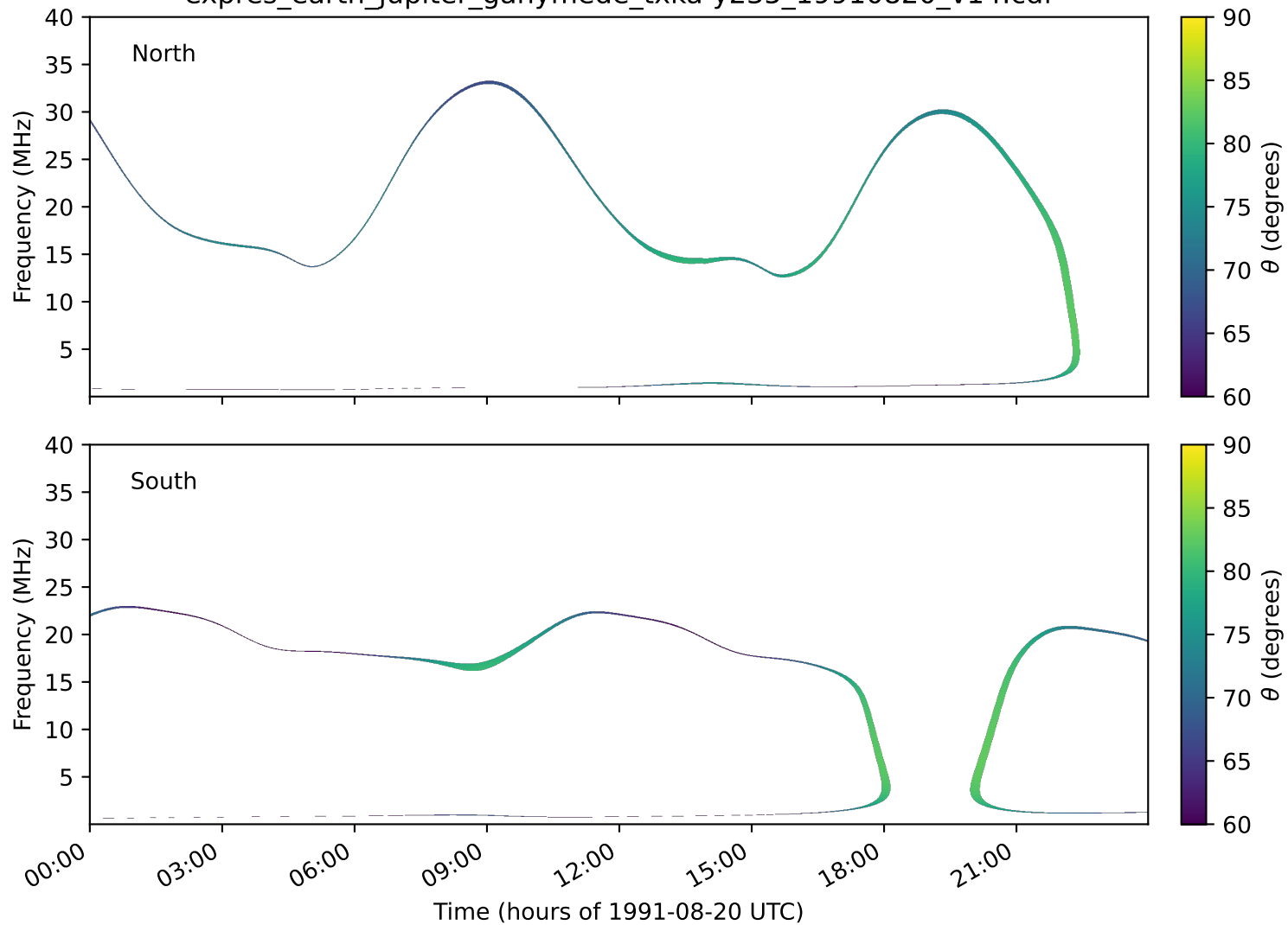
expres_earth_jupiter_ganymede_txka-y235_19910820_v14.cdf
