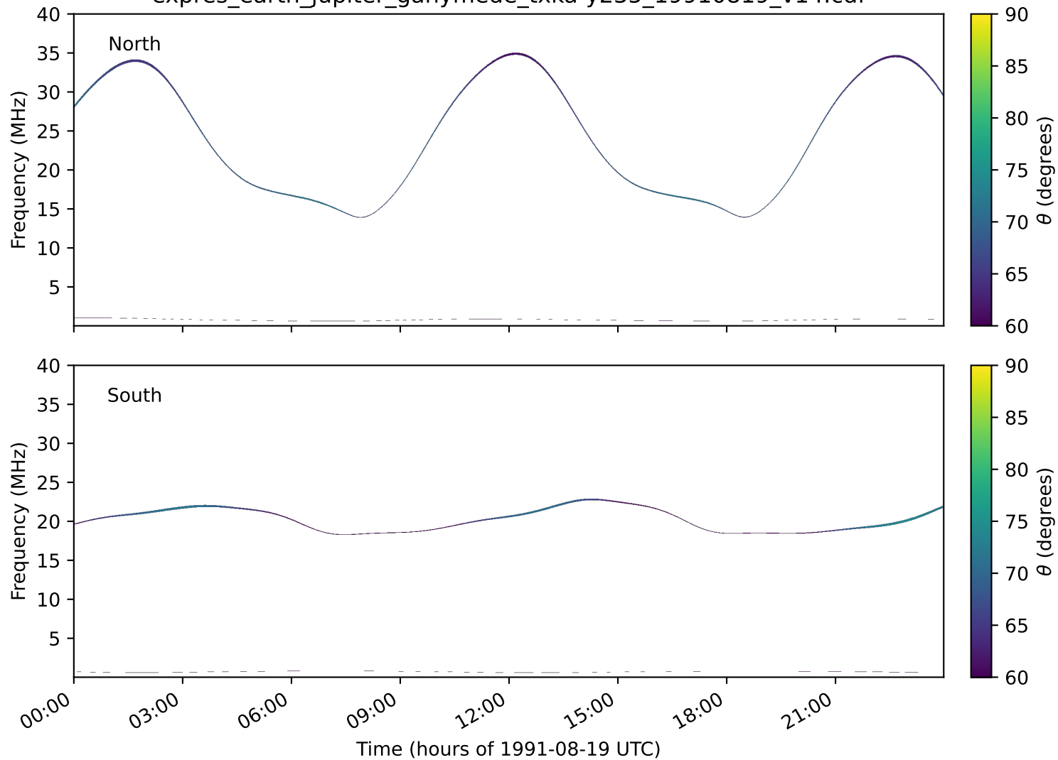
expres_earth_jupiter_ganymede_txka-y235_19910819_v14.cdf
