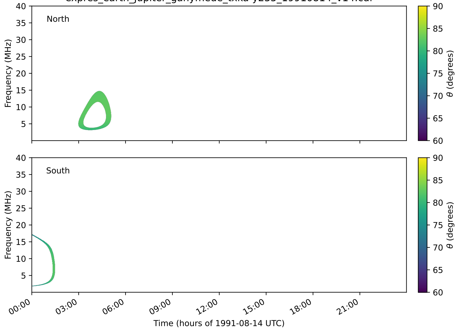
expres_earth_jupiter_ganymede_txka-y235_19910814_v14.cdf
