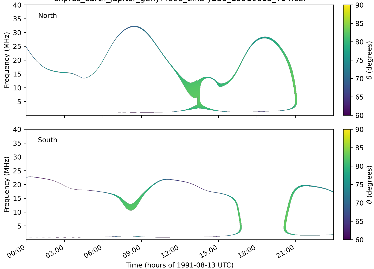
expres_earth_jupiter_ganymede_txka-y235_19910813_v14.cdf
