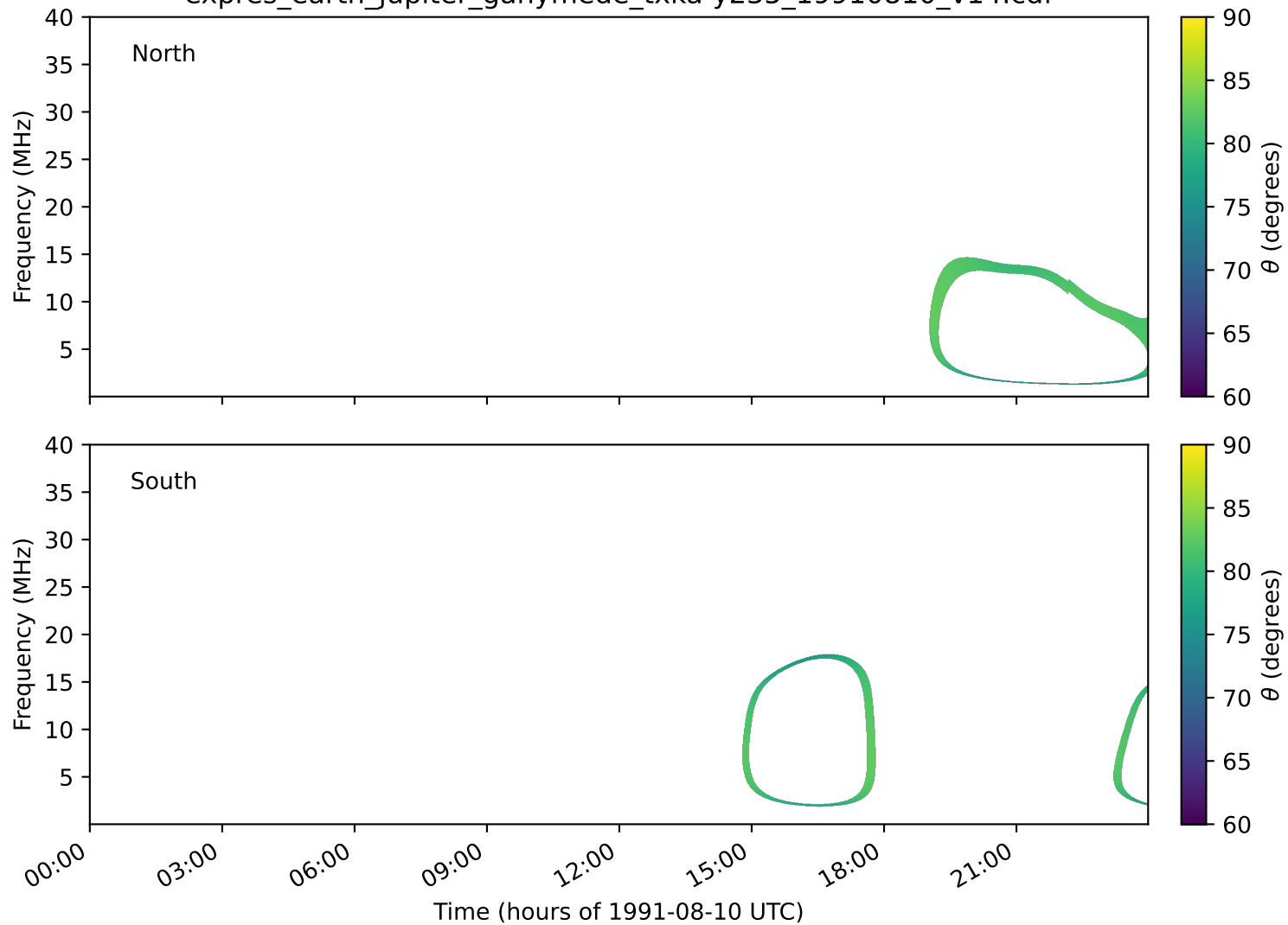
expres_earth_jupiter_ganymede_txka-y235_19910810_v14.cdf
