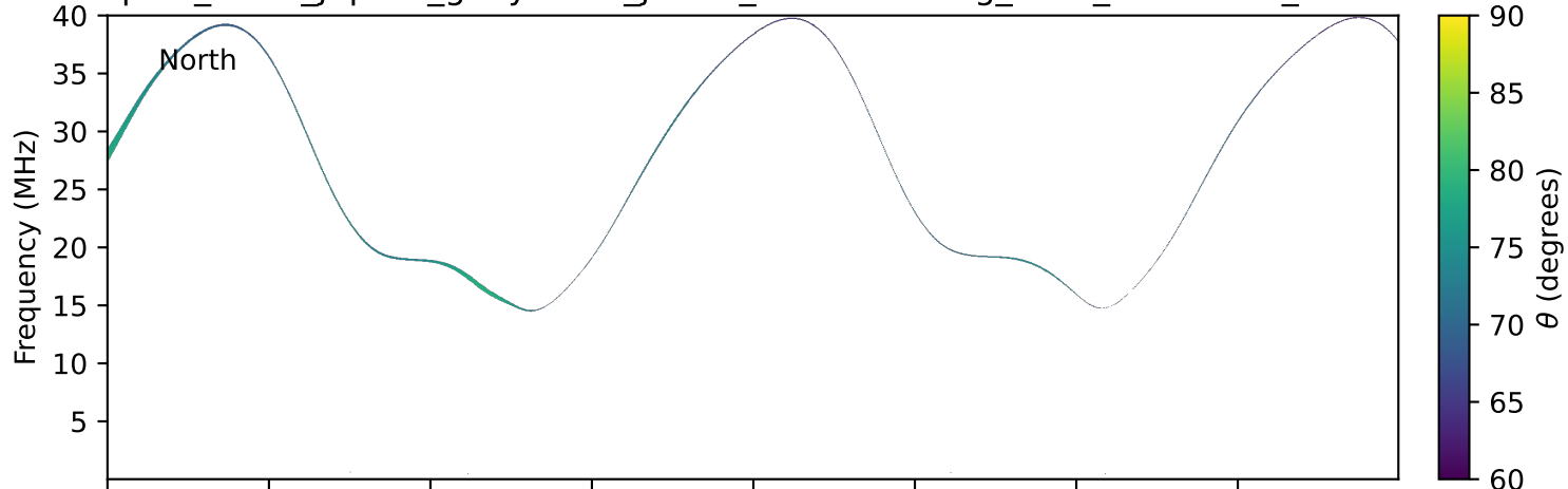
expres_earth_jupiter_ganymede_jrm33_lossc-wid1deg_3kev_19910826_v11.cdf
